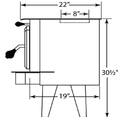
TOP-VENT SIDE VIEW
