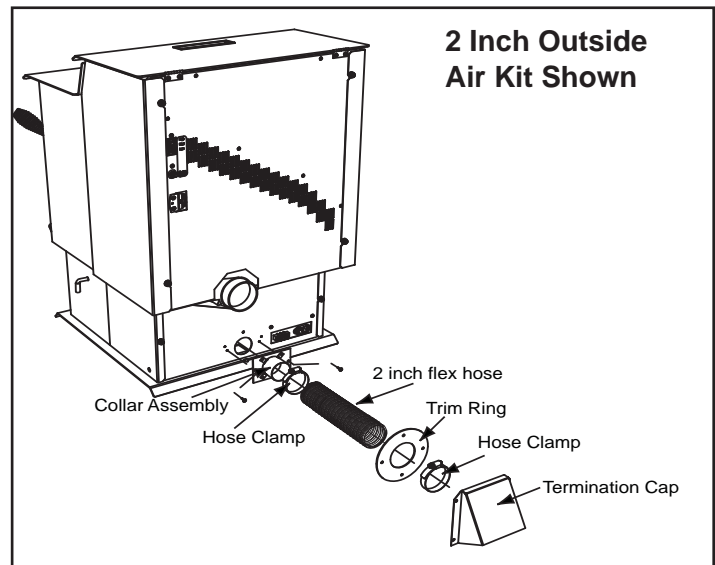
Figure 21.1 - 2 Inch Outside Air Kit
